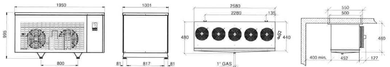
ICEBERG 100240SB
