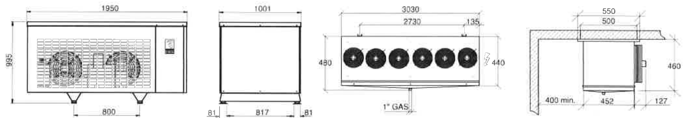
ICEBERG 50240SN
