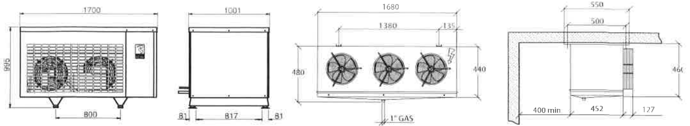
ICEBERG 30240SN
