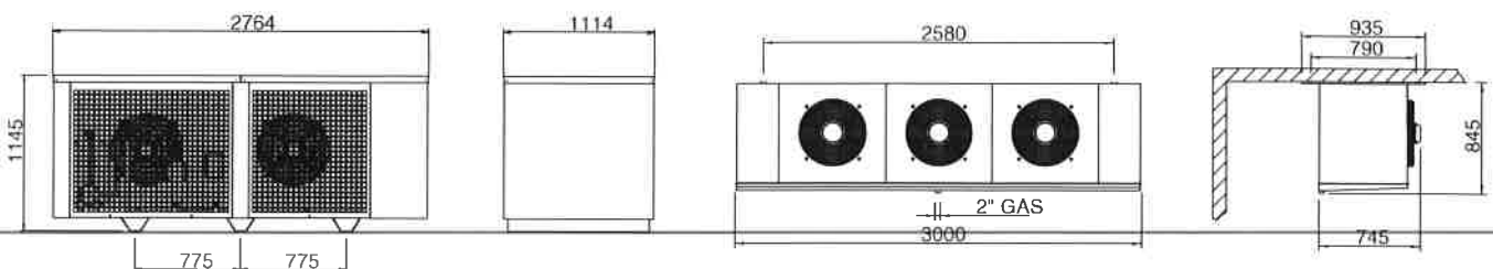
ICEBERG 200350N
