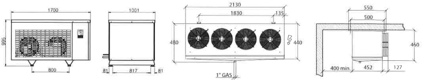
ICEBERG 40240SN
